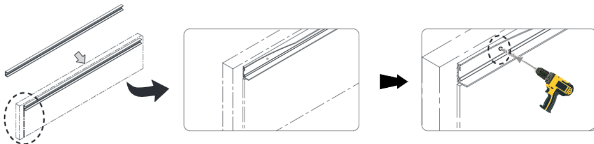
Figure 12: Proper installation of LEDs into U-channel.
