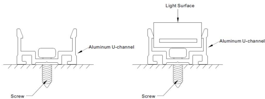
Figure 12: Proper installation of LEDs into U-channel.
