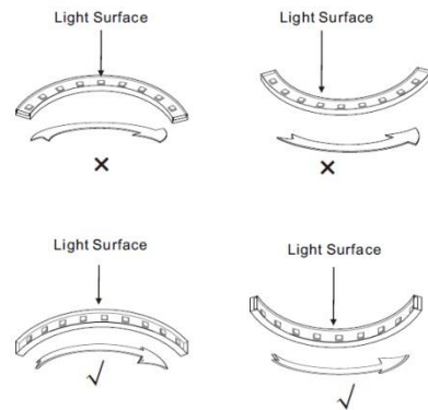
Figure 3: Only bend super flat rope light in the recommended directions.
