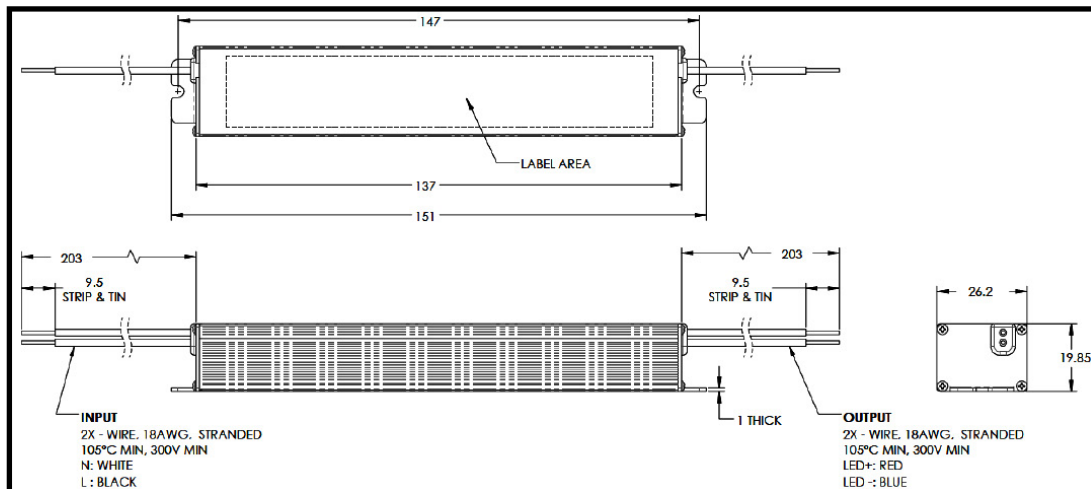
VLM100W-24
