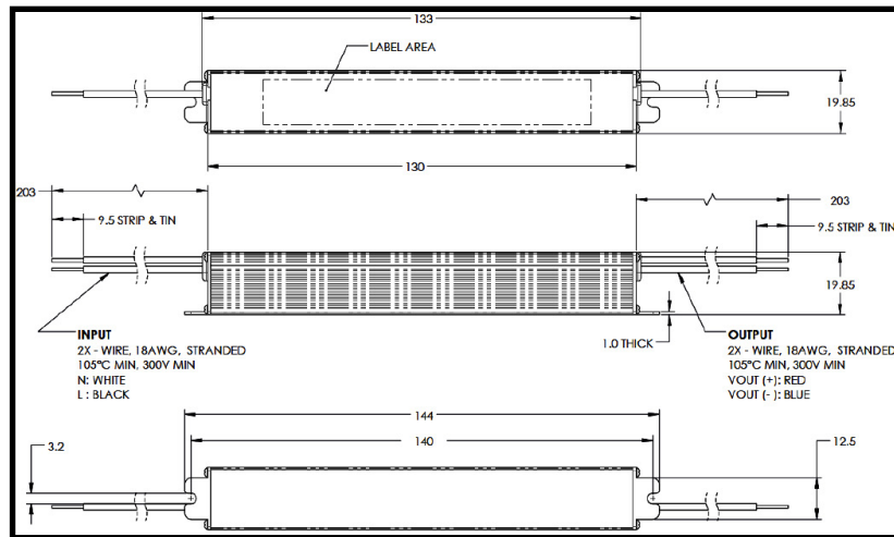
VLM60W-12
