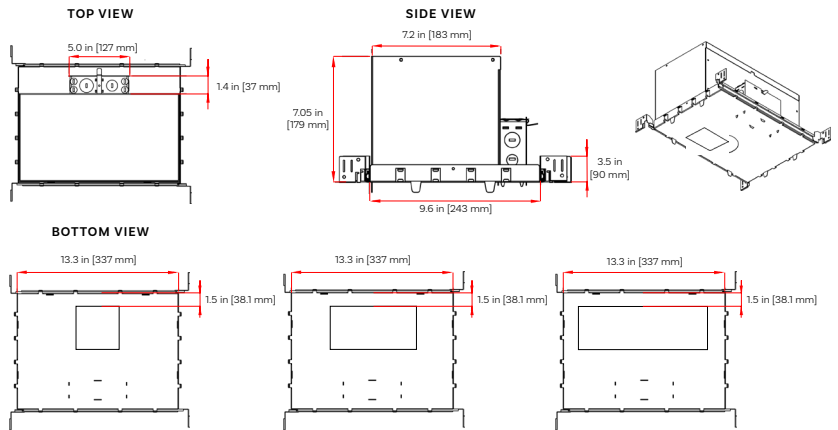
REVI 3-inch IC Rated Box, Square Double** REVI-IC3-S2
