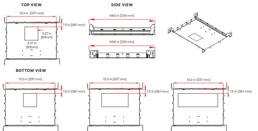
REVI 3-inch IC Rated Box, Square Double** REVI-FF3-S2
