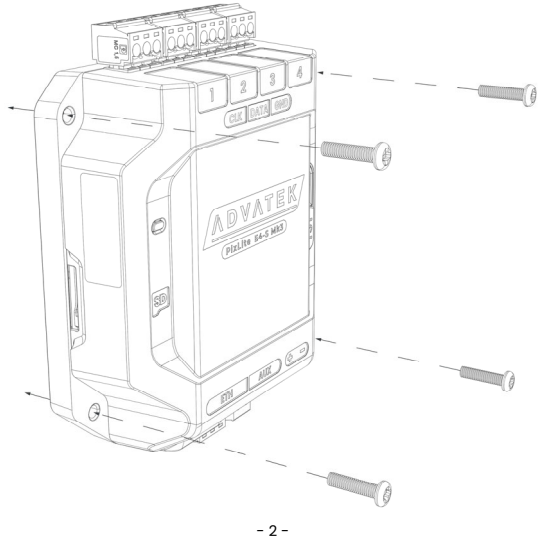
Figure 2: Controller Assembled to Wall
