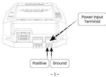
Figure 1: Location of Power Input
