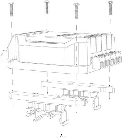
Figure 3: Controller Assembled to Bracket
