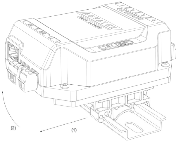
Figure 5: Removal of Controller from DIN Rail
