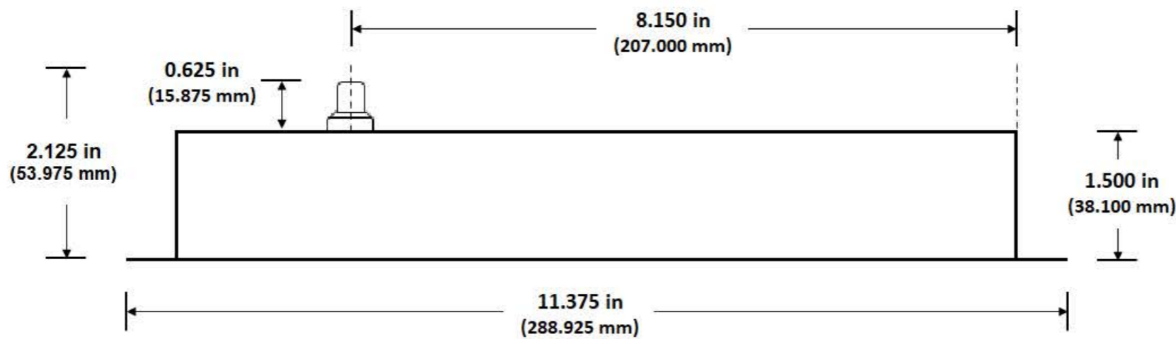
SIDE VIEW
