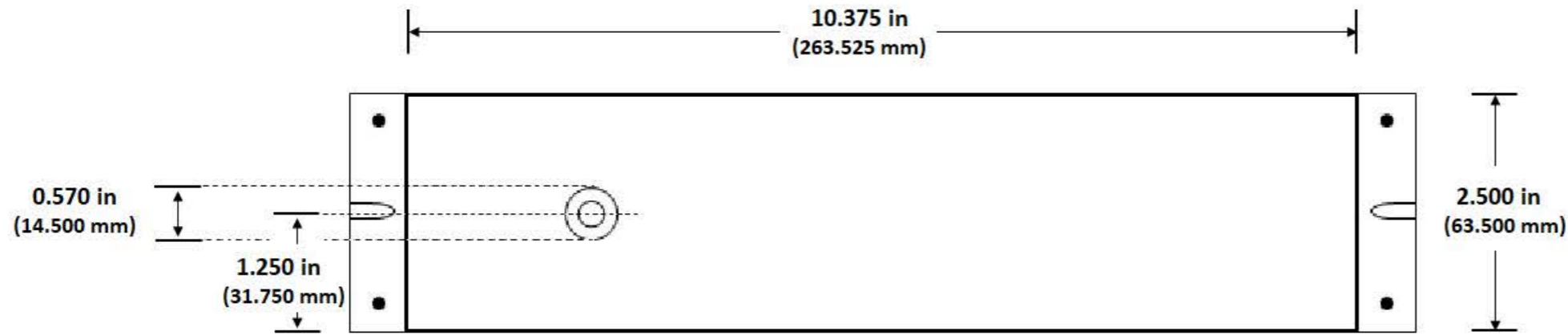
TOP VIEW
