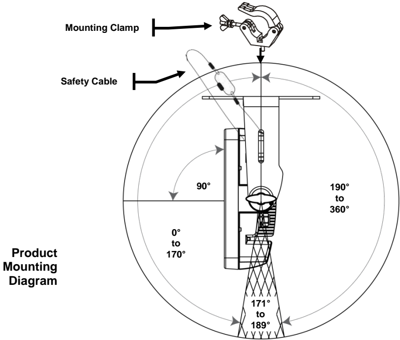
Overhead Mounting
