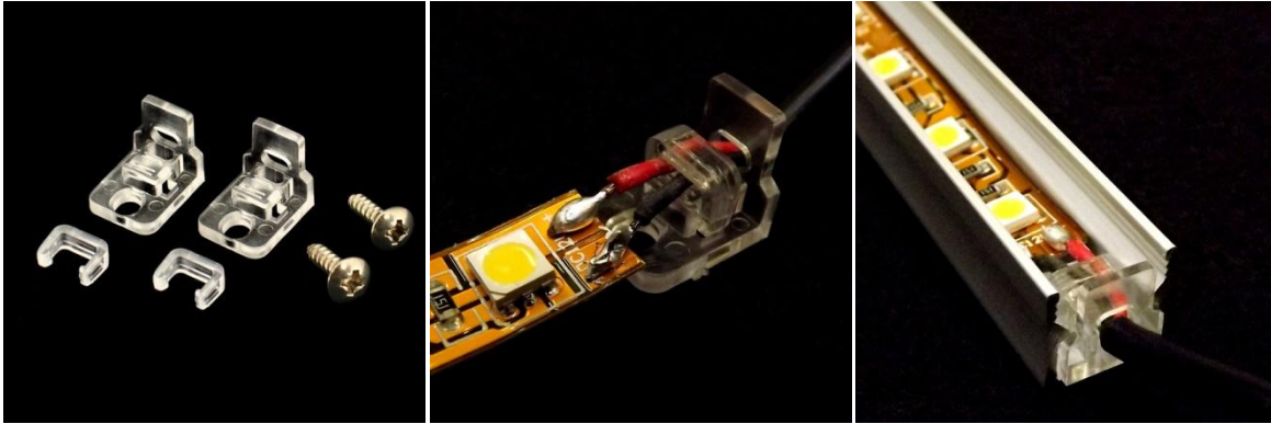
Aluminum Track End Clips led-track-clips
